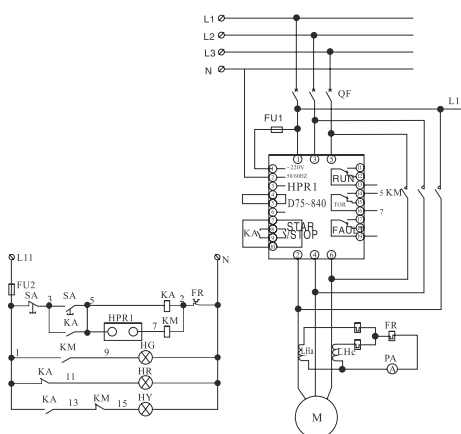
BQXR-37~90kW 电气原理图 Electrical principle chart
