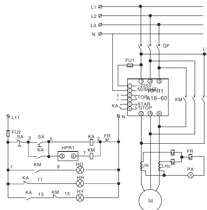
BQXR-7.5~30kW 电气原理图 Electrical principle chart
